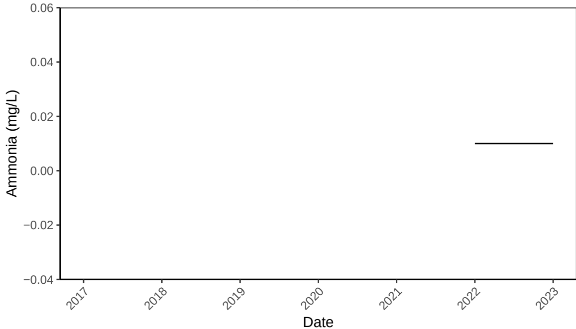
B2 Raceway 1 Ammonia (mg/L) Yearly Mean
